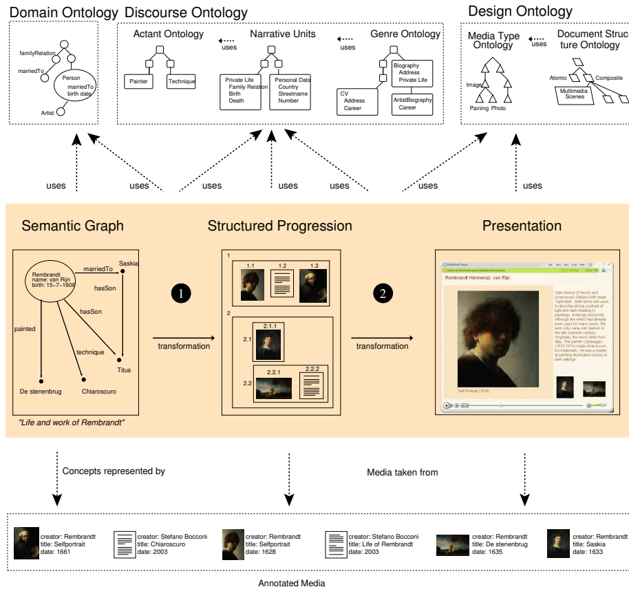
Fig.2. Sketch of the processing of the example scenario. The middle layer shows an example semantic graph (left) that is first transformed to a biography structure (middle) and then to a multimedia presentation (right). The upper layer shows the ontologies involved, while the lower layer represents the annotated media items used.
